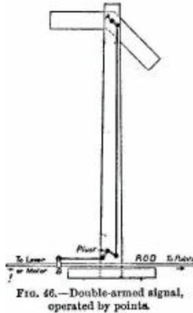
Fig. 46. -- Double-armed signal, operated by points.
