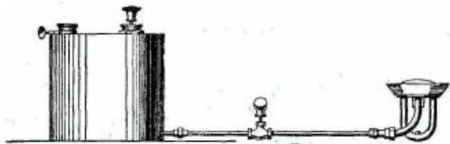
FIG. 95.—Paraffin burner for vertical boiler.
