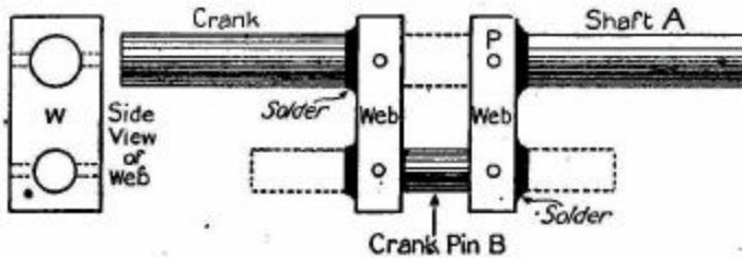
FIG. 101.—Details of built-up crank.
