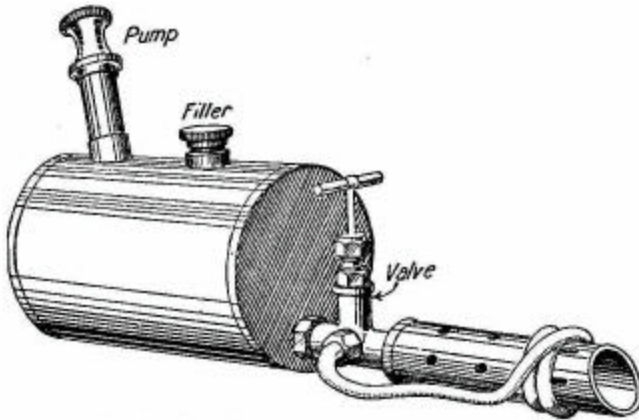
FIG. 94.—Benzoline lamp for model central-flue boiler.
