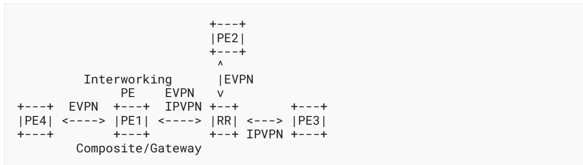
Figure 3: Interworking Composite/Gateway PE Example
